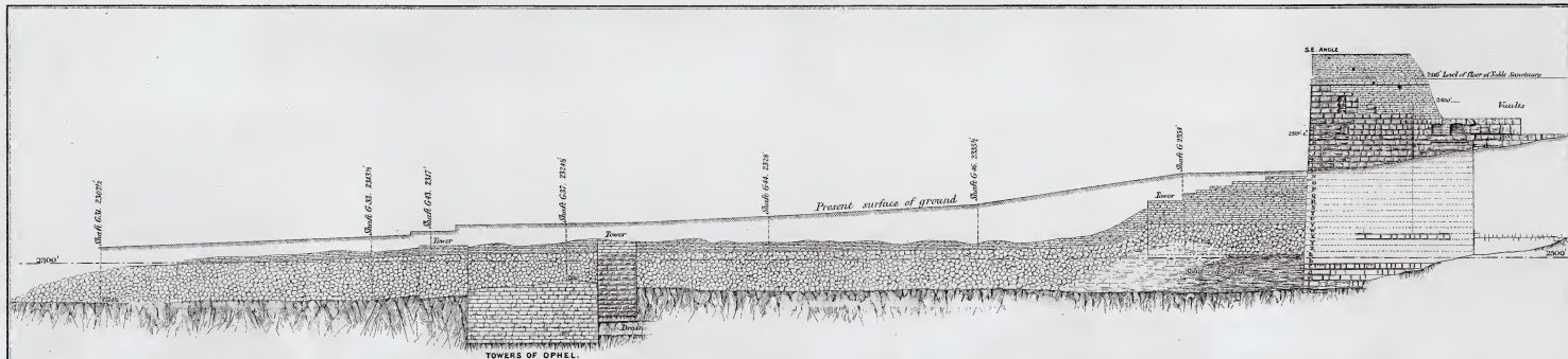
ELEVATION OF OPHEL WALL FROM EAST.
